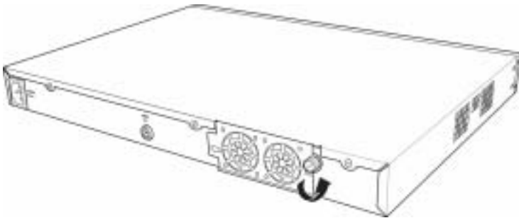
Figure 54. Loosening the thumbscrew
